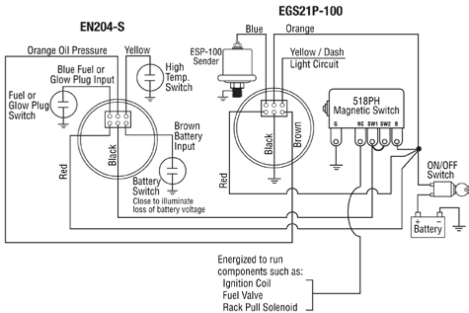
EN204-S Typical Wiring Diagram
