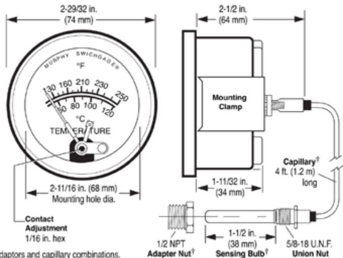
A25 Series Models (typical)
