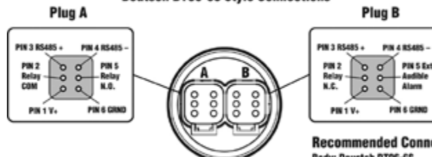
PowerView Audible Alarm Back View Deutsch DT06-6S Style Connections
