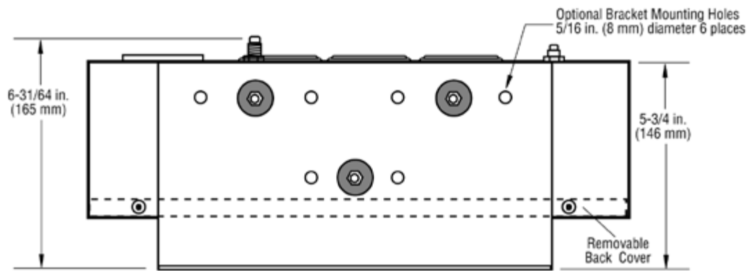
Bottom View
