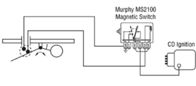
Typical Wiring for LR589
