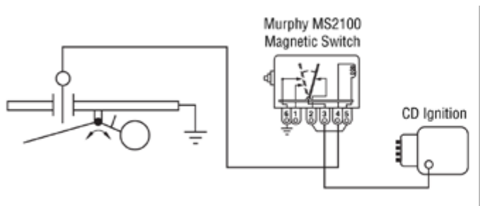
Typical Wiring for LR579
