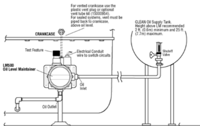
Pipe Mount
