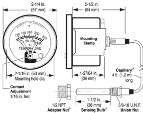
A20 Series Models (typical)
