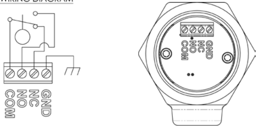
STD WIRING DIAGRAM
