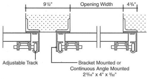
2" Track
