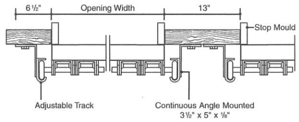
3" Track
