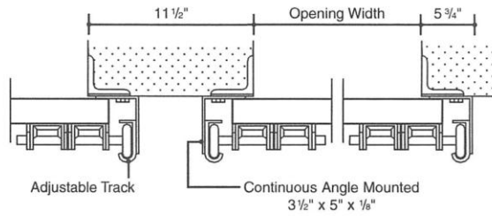
3" Track
