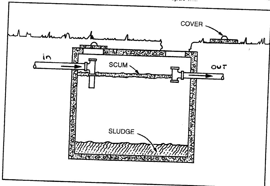
Cross section of a typical ventless septic tank
